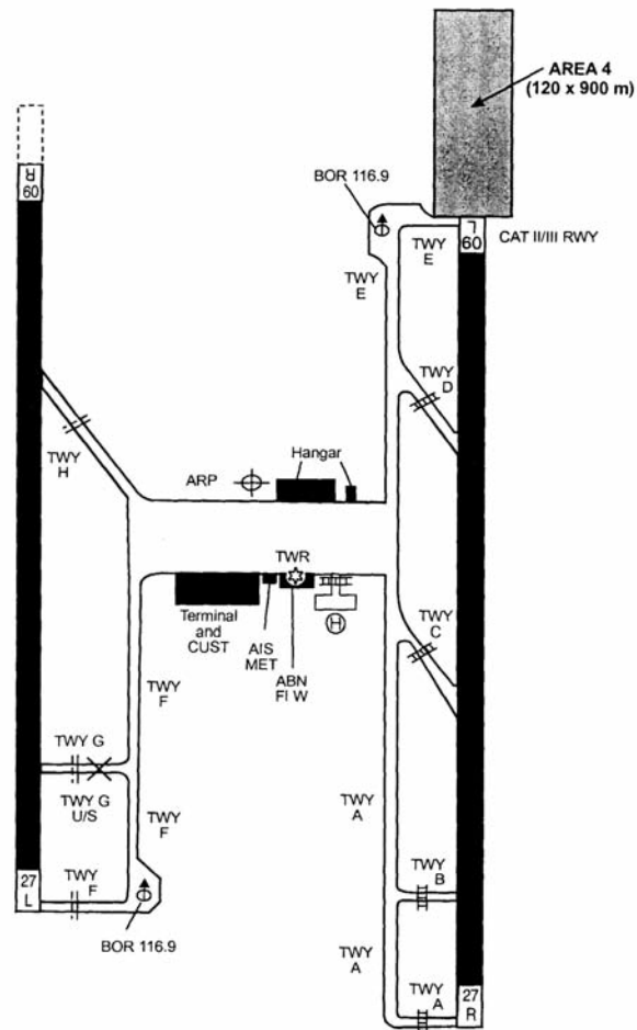
Figure A8-4. Terrain data collection surface — Area 4
