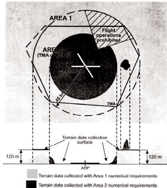
1 Figure 1 Terrain data collection surfaces — Area 1 and Area 2
