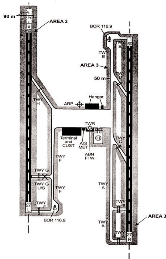
Figure 3. Terrain and obstacle data collection surfaces—Area 3
